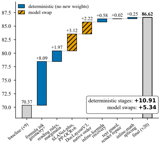
OmniDocBench v1.6 Overall (axis starts at 68, not 0)
