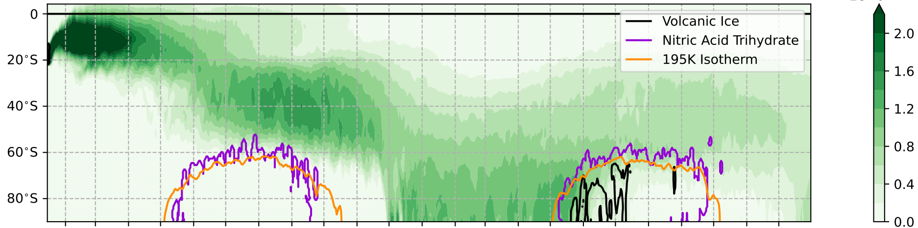
Tagged Volcanic Total Surface Precipitation Rate (mm/day)
