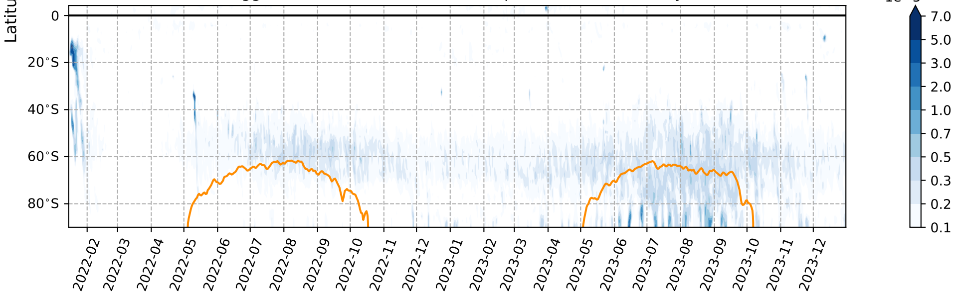
Tagged Volcanic Total Surface Precipitation Rate (mm/day)
