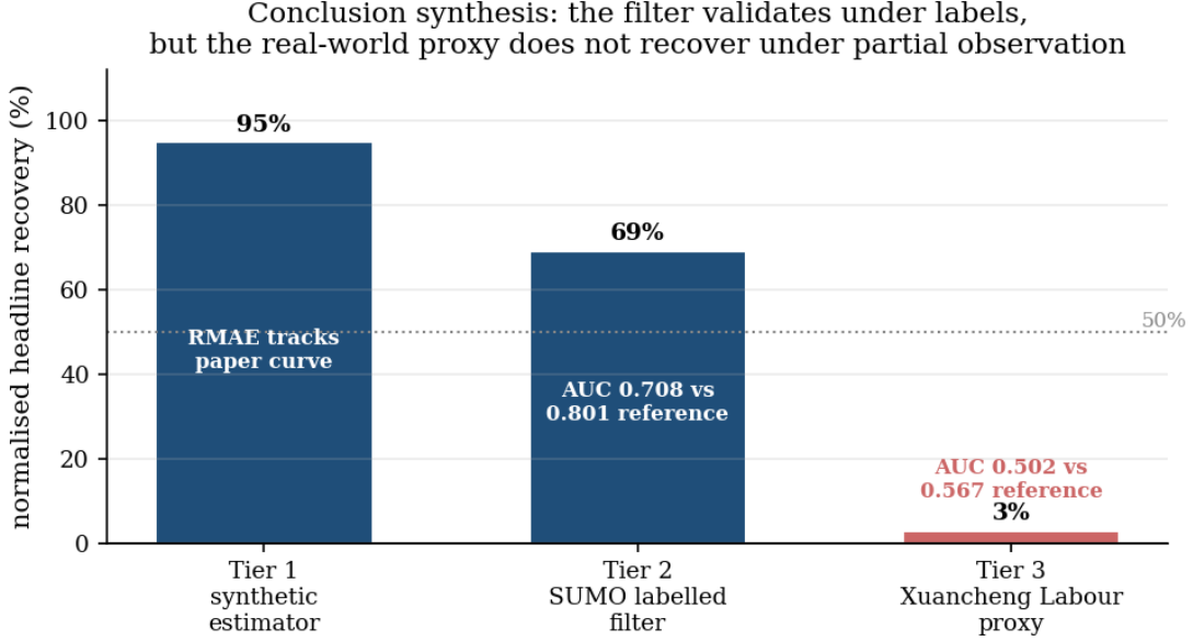
Figure 7: Cross-tier synthesis of the dissertation’s headline results. The bars use a normalised summary, since the tiers use different metrics: Tier 1 reports benchmark-reproduction closeness, computed as the mean capped ratio between the visual paper RMAE and this reproduction’s RMAE for |X_o| \geq 10 ; Tiers 2–3 report AUC gap closed, (AUC_{\text{fit}} - 0.5)/(AUC_{\text{emp}} - 0.5) . The central pattern is that the estimator reproduces its synthetic benchmark, the labelled SUMO filter recovers a substantial fraction of the empirical 1-step signal, and the real Xuancheng behavioural proxy does not recover under the fitted partial-observation model.
