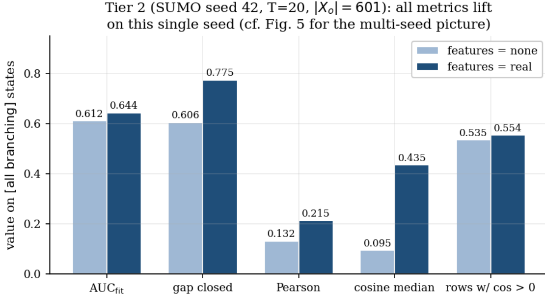
Figure 1: Tier 2 features lift on the Ingolstadt SUMO network, seed 42, T = 20 . Every metric, including detection AUC, gap-closed, per-row Pearson, per-row cosine median and fraction of rows with positive cosine, moves positively under features=real (dark) vs. features=none (light). The Pearson +63% relative lift and the cosine median 4.6× lift on the [all branching] generalisation block are the strongest evidence that chain recovery, not aggregate-bias drift, is what features improve.
