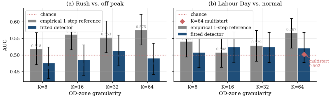
Figure 5: Tier 3 OD-matched proxy sweeps. (a) In the rush-vs-off-peak proxy, the empirical reference returns above chance for K \geq 16 , but the fitted detector stays near chance. (b) Labour Day creates the clearer empirical contrast at K = 64 , yet the fitted detector remains weak and the validation-selected multistart result drops to 0.502. Error bars are bootstrap 95% confidence intervals for the shown AUCs.
