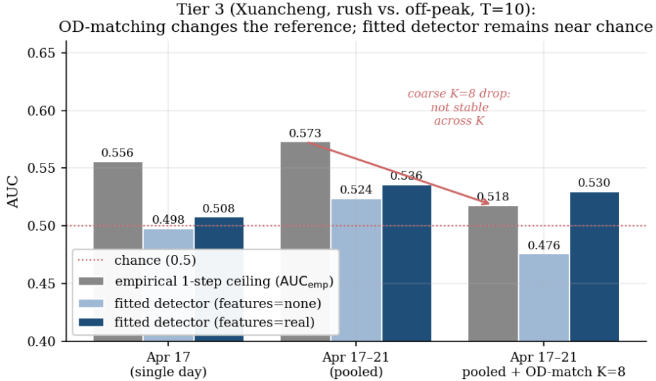
Figure 4: Tier 3 Xuancheng rush-vs-off-peak detection AUC across three configurations. The full-observation empirical 1-step reference (grey) is 0.556 on a single day, 0.573 when 5 weekdays are pooled, and 0.518 once the pools are OD-matched at K = 8 spatial zones. The apparent crash at K = 8 is not stable across zone granularity: a sweep over K \in \{8, 16, 32, 64\} (table 8) shows the matched reference returning to \sim 0.55 – 0.58 for K \geq 16 . The K = 8 drop is therefore not treated as a fixed OD-mix fraction. Fitted detectors (blue bars) sit at or below chance in all three configurations.
