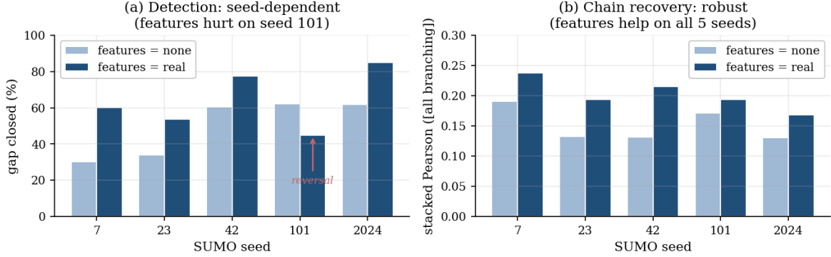
Figure 2: Multi-seed Tier 2 features sweep (five SUMO seeds, [all branching] block, T=20 ). (a) The aggregate detection metric (gap-closed) lifts under features=real on four seeds but reverses on seed 101; the features=none bars also reproduce the bimodal basin structure ( \{7, 23\} low, \{42, 101, 2024\} high). (b) The per-row chain-recovery metric (stacked Pearson) lifts on all five seeds. Features are a robust chain-recovery lever, not a robust aggregate-detection lever.
