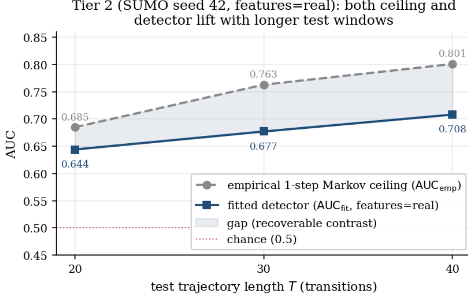
Figure 3: Tier 2 T -sweep on the Ingolstadt SUMO network, seed 42, features=real . The empirical 1-step Markov reference (grey dashed) rises with T as expected for a variance-shrinking score; the fitted detector (blue solid) tracks it with roughly constant gap. The shaded region is the recoverable contrast not yet captured by the fitter. The fitted chain itself is T -independent (identical final losses across runs); only the trajectory-level scoring window changes.
