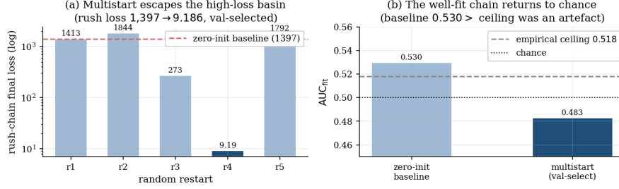
Figure 6: Xuancheng OD-matched features=real multistart ( K=5 ). (a) The rush-chain training loss collapses from the zero-init baseline (1,397) to the validation-selected restart (9.186): random re-initialisation escapes the high-loss basin, unlike the SUMO case (section E). (b) Despite the proper fit, AUC_{fit} falls from the baseline’s spurious 0.530 (which exceeded the empirical ceiling 0.518) to 0.483 – chance. The ceiling violation was an optimiser artefact; under correct chain recovery the fitted detector returns to chance.
