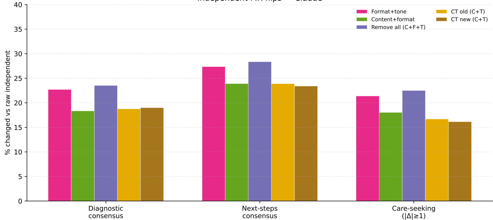
Independent MR flips — Claude
