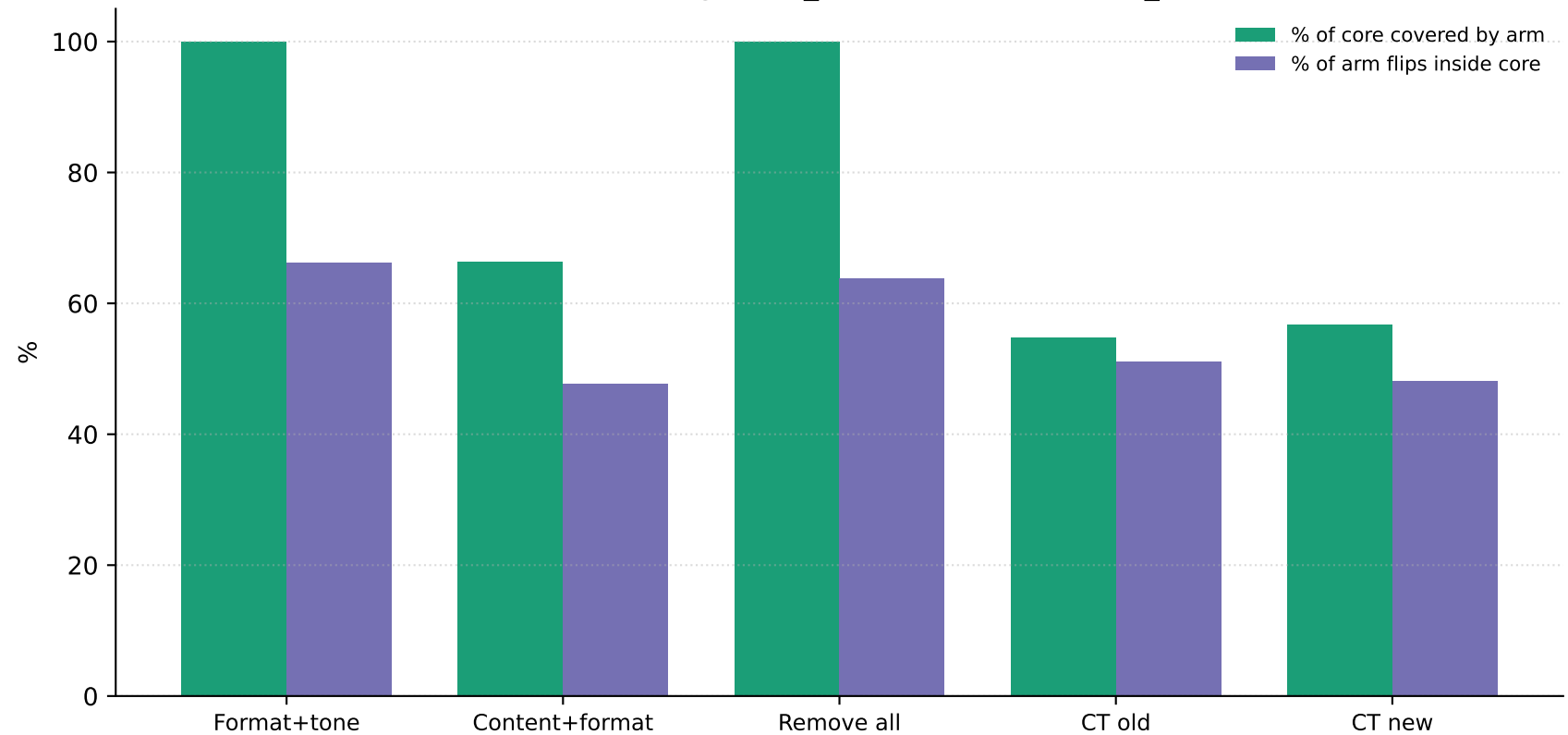
Gemini — diagnostic_consensus vs core=ra_ft
