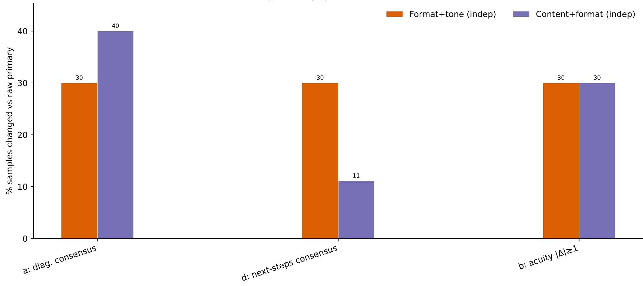
Answer change rate by question and ablation (Claude)
