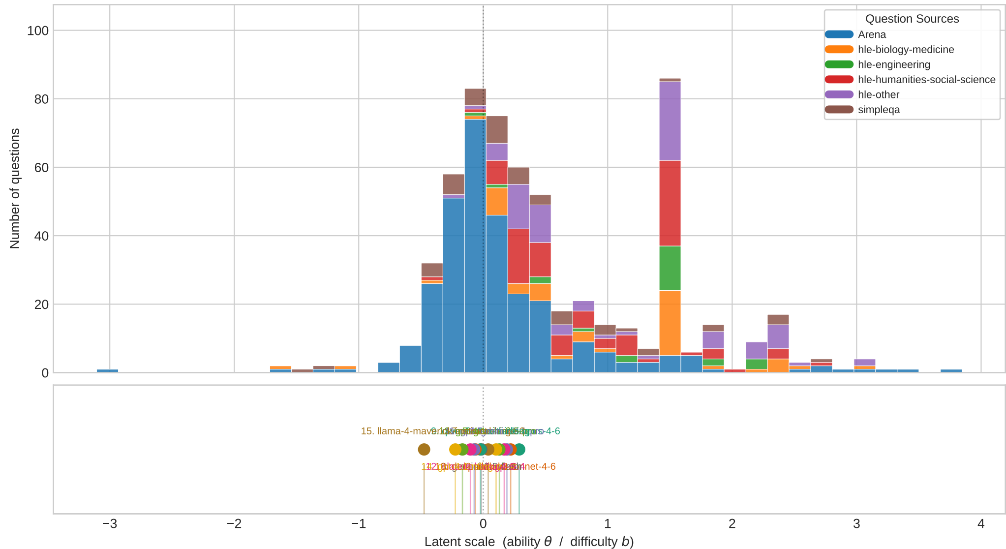
Pairwise+Regression IRT Ranking (v1)
