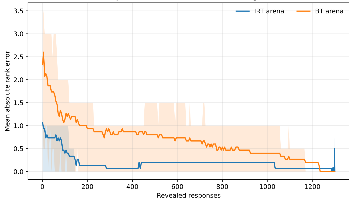
Adaptive Arena Cold-Start Rank Convergence
