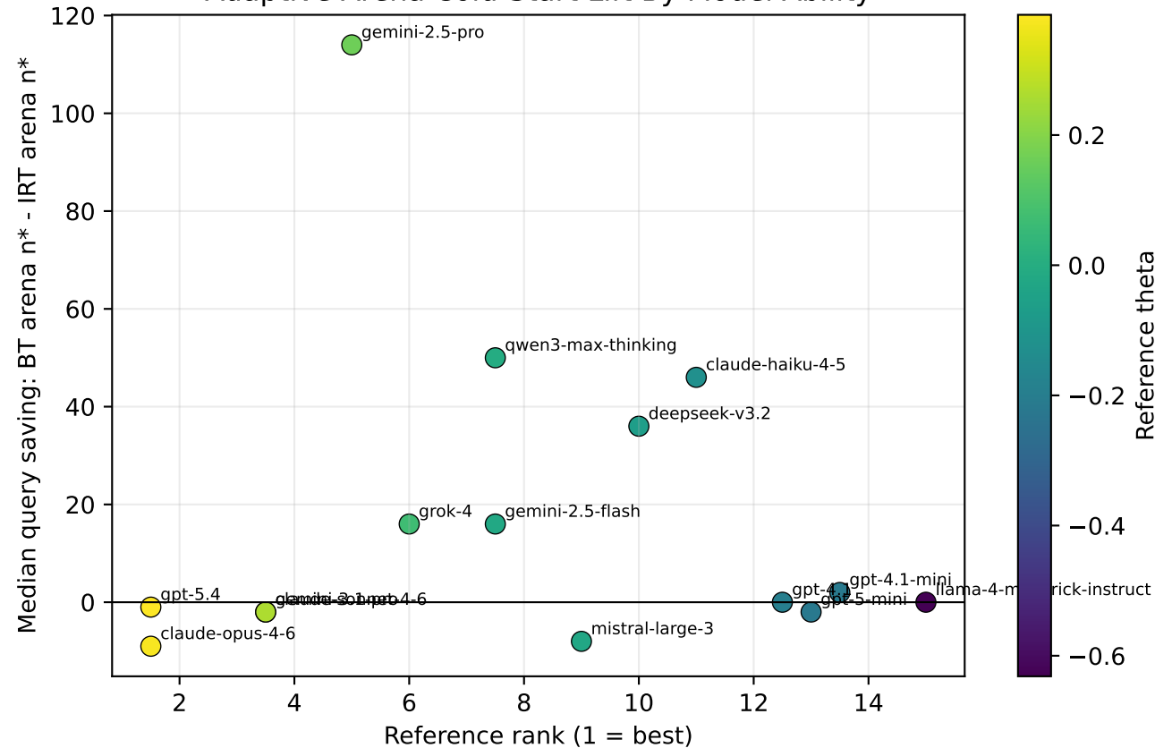
Adaptive Arena Cold-Start Lift By Model Ability
