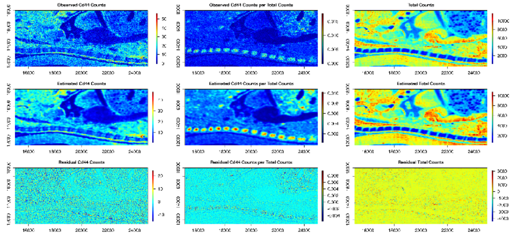
Fig 3. Raw vs. count-normalized topology. Example comparison between raw count topology vs. count-normalized topology for a single feature (Cd44). 1 st column is observed Cd44 counts, 2 nd column is observed Cd44 counts divided by the total counts. 3 rd column is the total counts. 1 st row is raw data, 2 nd row are estimates from the spatial model, 3 rd row is the residual (difference between model and raw data.) In this example, count-normalization substantially changes the spatial topology. On this basis, and on the comparable panels for 23 further features in S3 File, we avoid normalization prior to connectivity computations in the work reported here.
