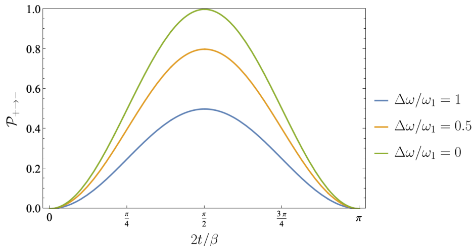
Figure 3.1: Probability for a spin flip to occur as a function of 2t/\beta , where \beta = \sqrt{\Delta\omega^2 + \omega_1^2} , for various values of \Delta\omega/\omega_1 . Near resonance, \Delta\omega = 0 , and the maximum probability is one.
