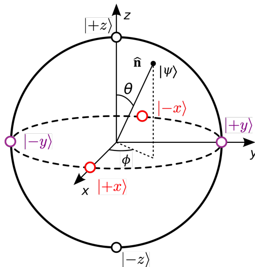
Figure 2.1: The Bloch sphere—a convenient way to visualize spin-1/2 systems. Any pure state can be mapped to some point on the Bloch sphere.
