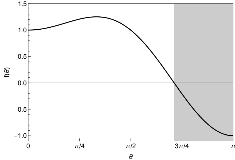
Figure 3.1: Plot of f(\theta) = 2r(\theta) - r(2\theta) . The shaded region marks angles for which f(\theta) < 0 , indicating violation of the local hidden-variable bound.
