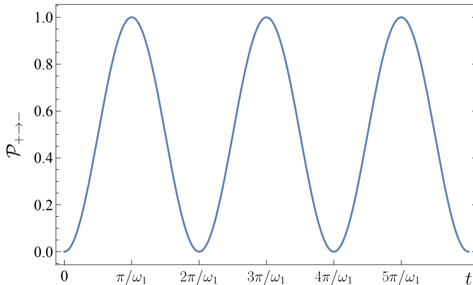
Figure 3.2: Rabi oscillations: probability for a spin-flip to occur over time when the driving field is resonant with the Larmor precession of the dipole.
