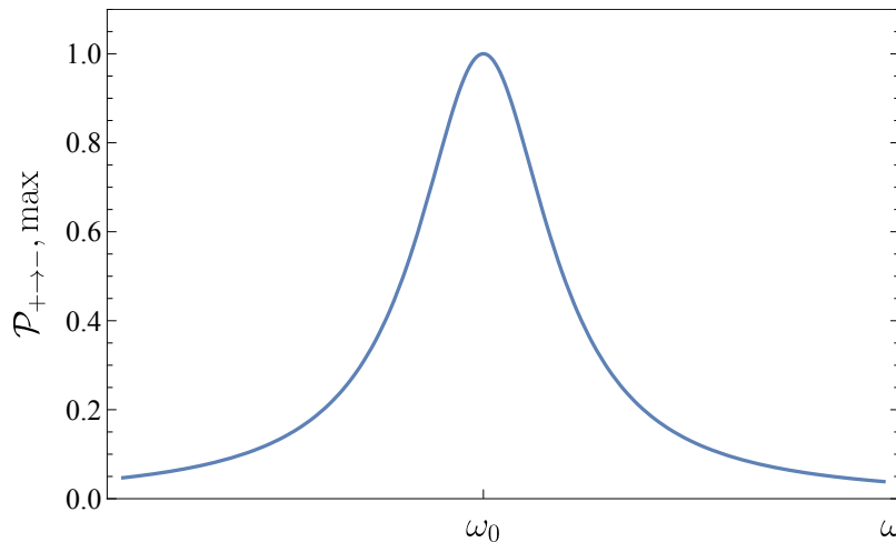
Figure 3.1: Magnetic resonance curve showing the maximum probability of a spin flip as a function of the applied frequency.
