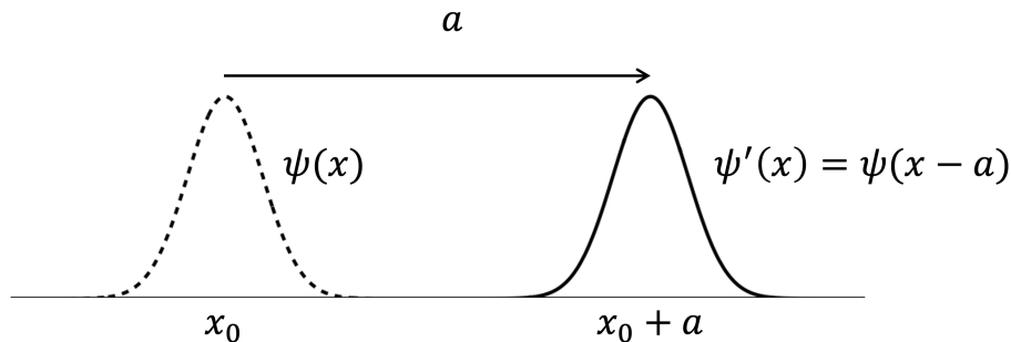
Figure 2.1: For a > 0 , the translation operator shifts the wave function to the right such that the new wave function \psi'(x) = T(a)\psi(x) = \psi(x - a) , at position x , takes the values of the old wave function \psi(x) at position x - a .
