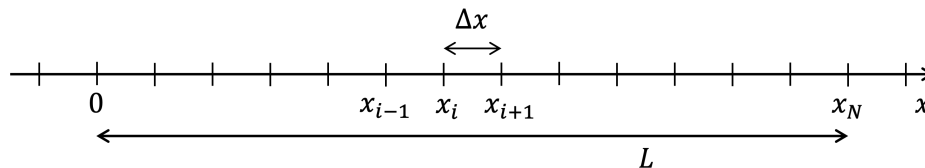
Figure 1.1: A particle moves on a line with a nonzero probability of being found within a region of length L . We discretize the allowed positions and then take a continuum limit.
