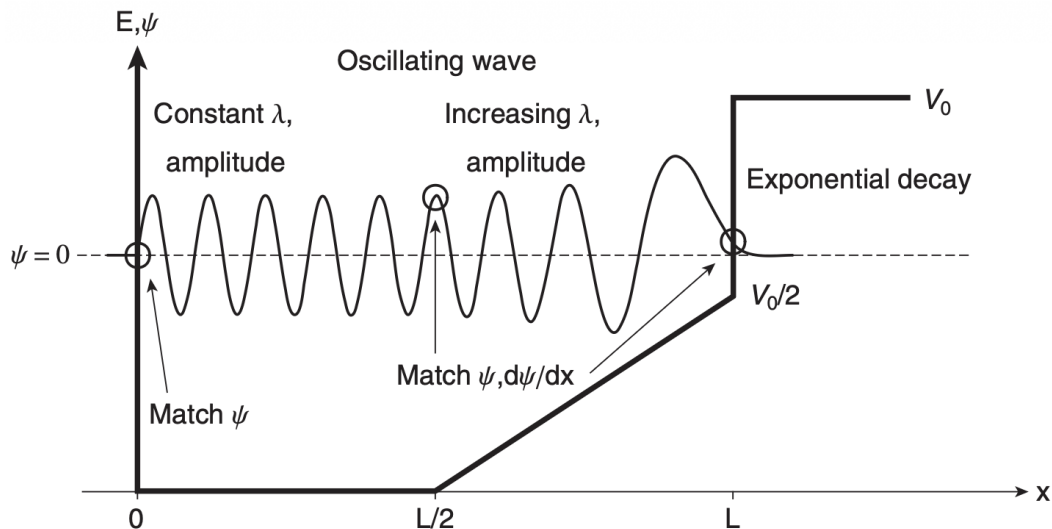
Figure 1.3: Drawing approximate energy eigenstate solutions. (McIntyre, 2022)
