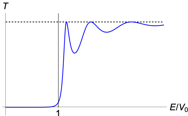
Figure 4.2: Transmission coefficient for scattering from a square barrier for V_0 = 12 in dimensionless units. Nonzero T for E < V_0 corresponds to quantum mechanical tunneling.
