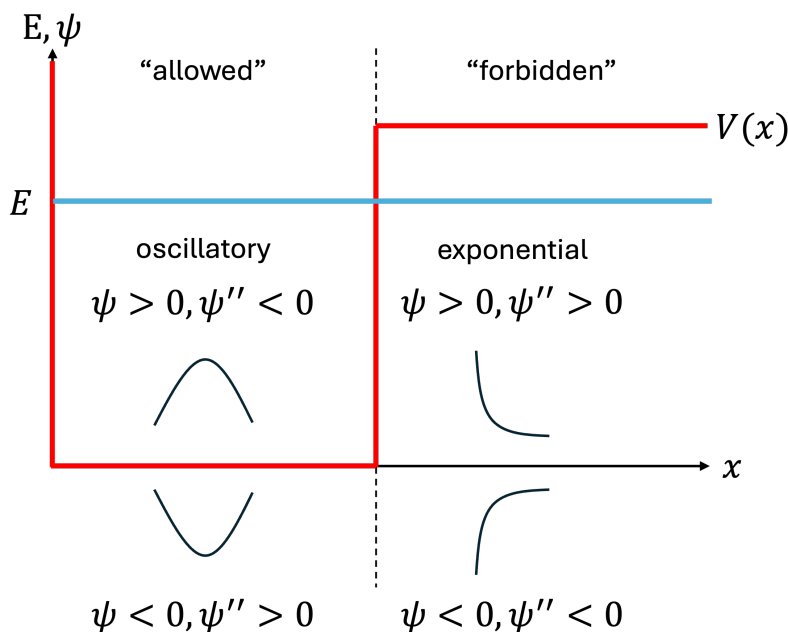
Figure 1.2: Curvature of the energy eigenstate wave functions in the allowed and forbidden regions.
