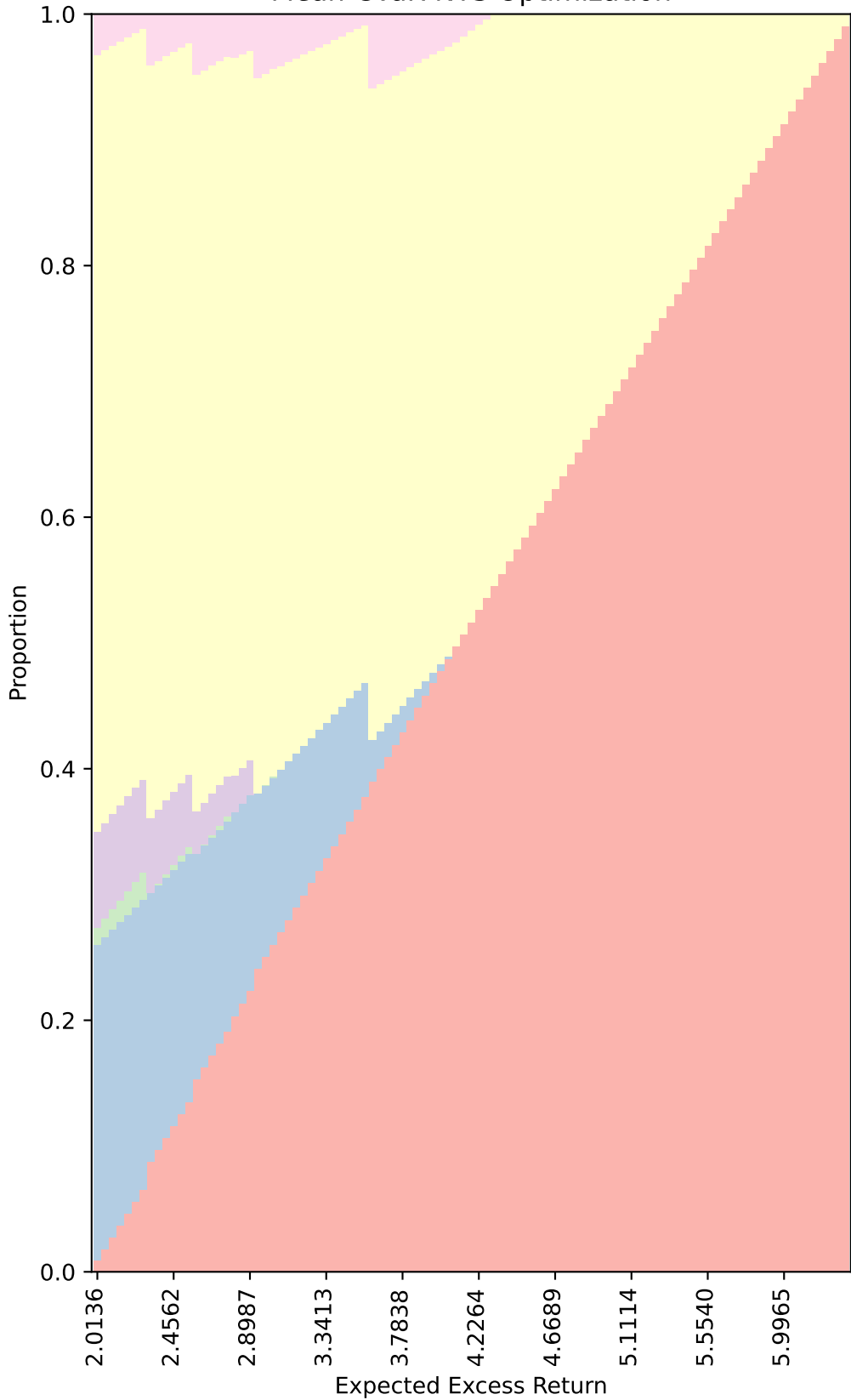
Mean-CVaR-NTS Optimization
