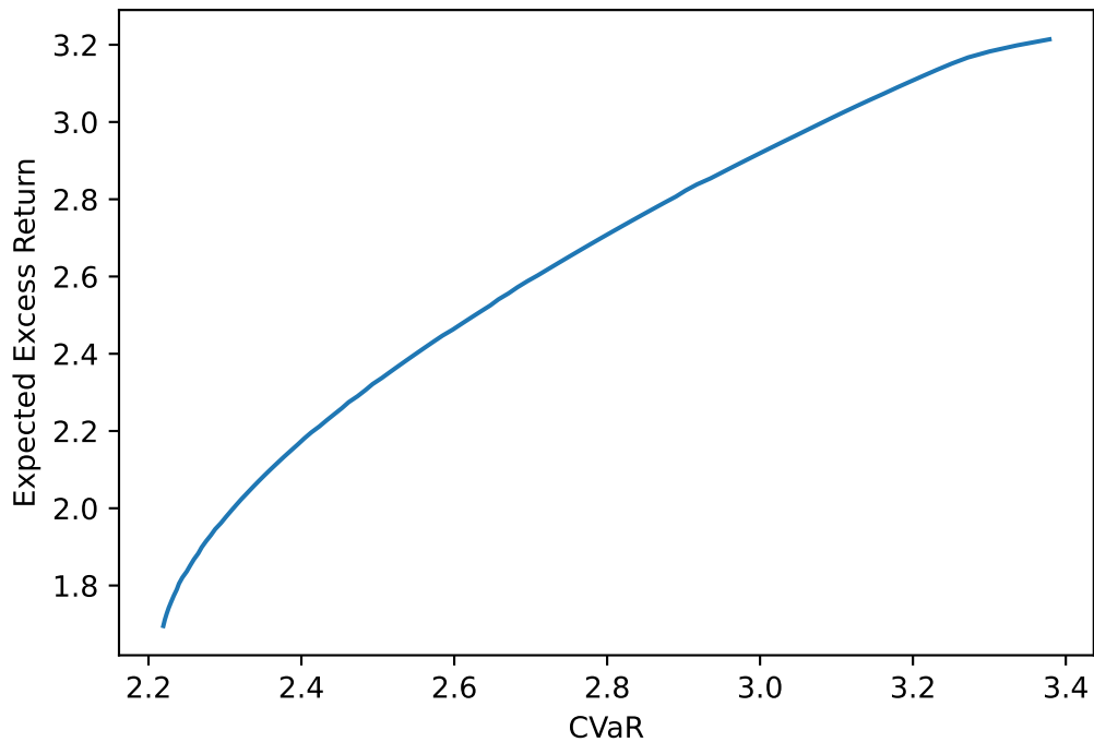
Mean-CVaR-NTS Optimization
