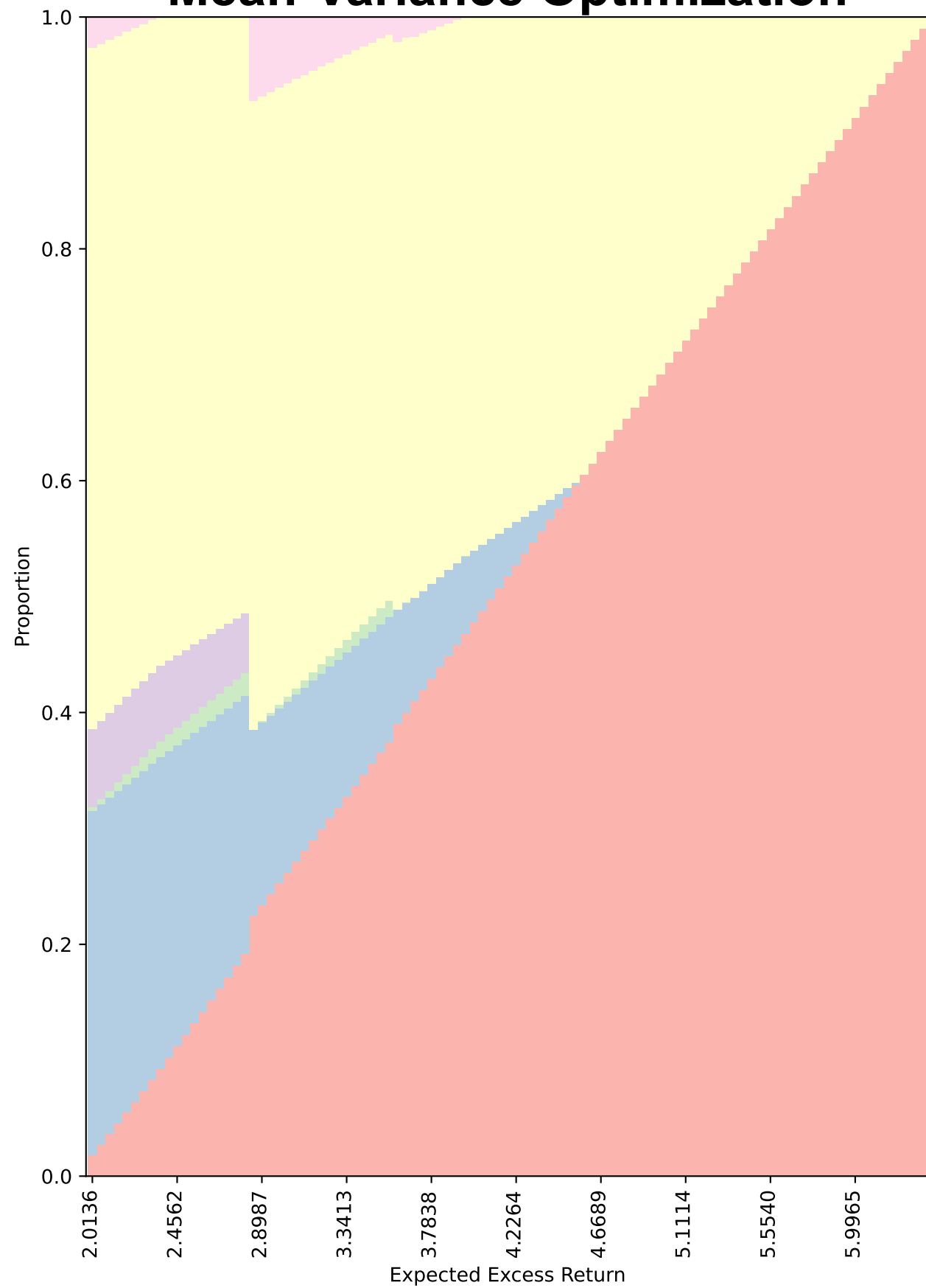
a1 Mean-Variance Optimization
