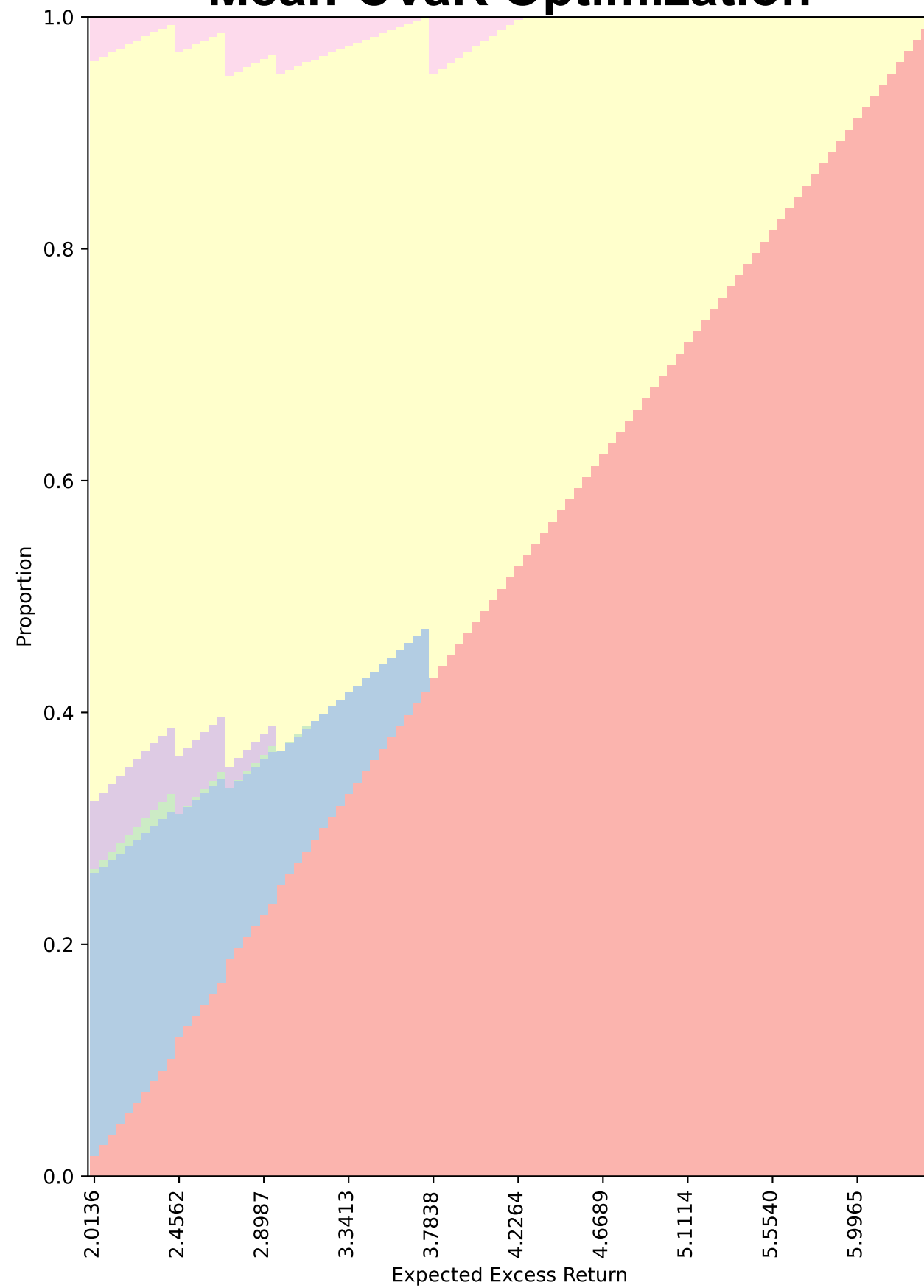
a2 Mean-CVaR Optimization
