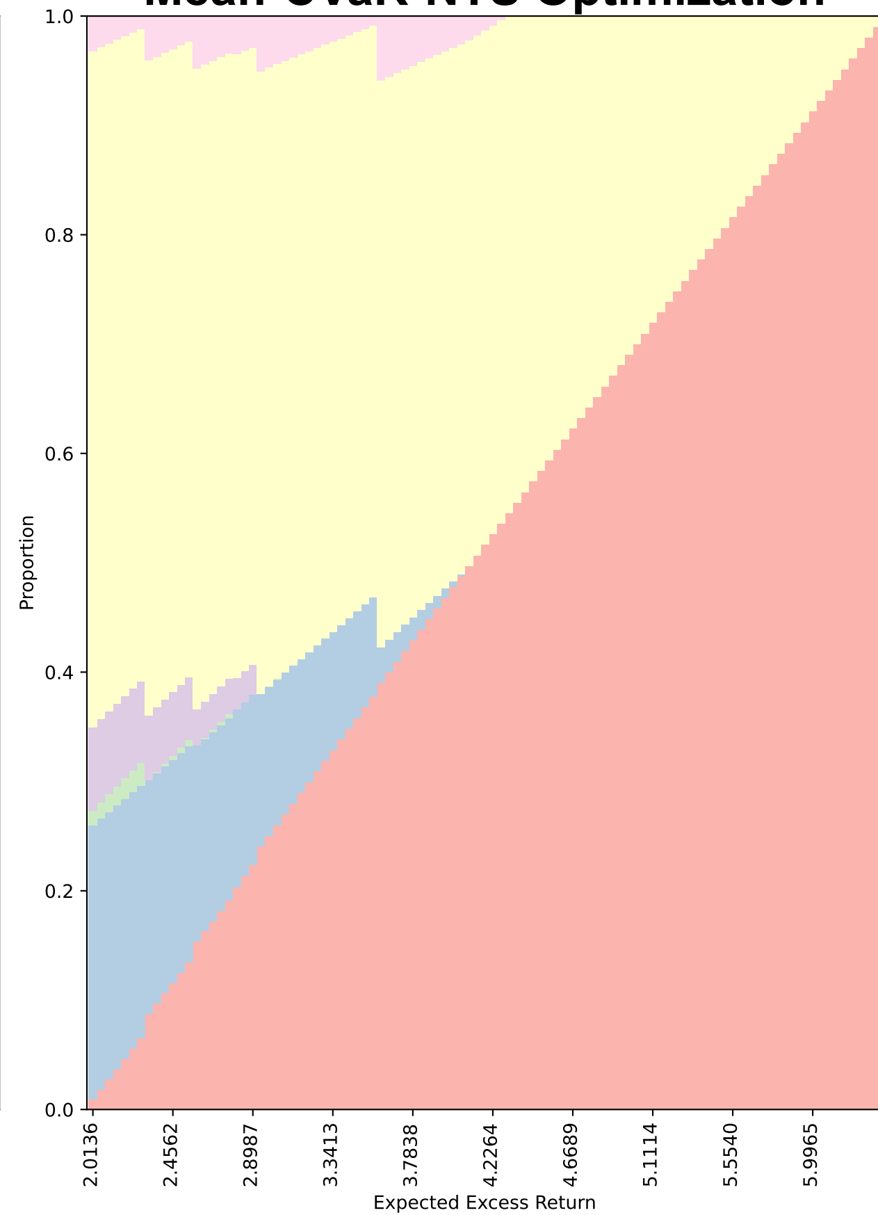
a3 Mean-CVaR-NTS Optimization
