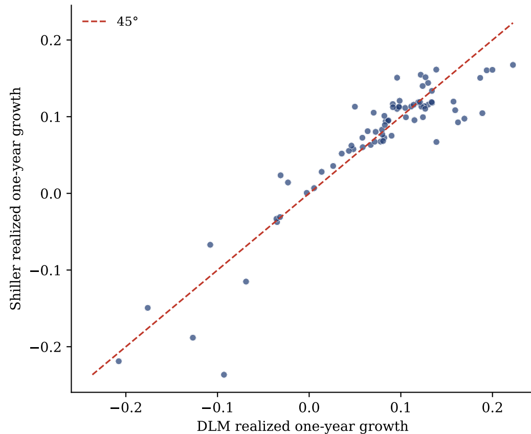
Dividends (corr = 0.919, n=75)
