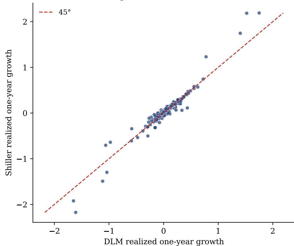
Earnings (corr = 0.969, n=183)
