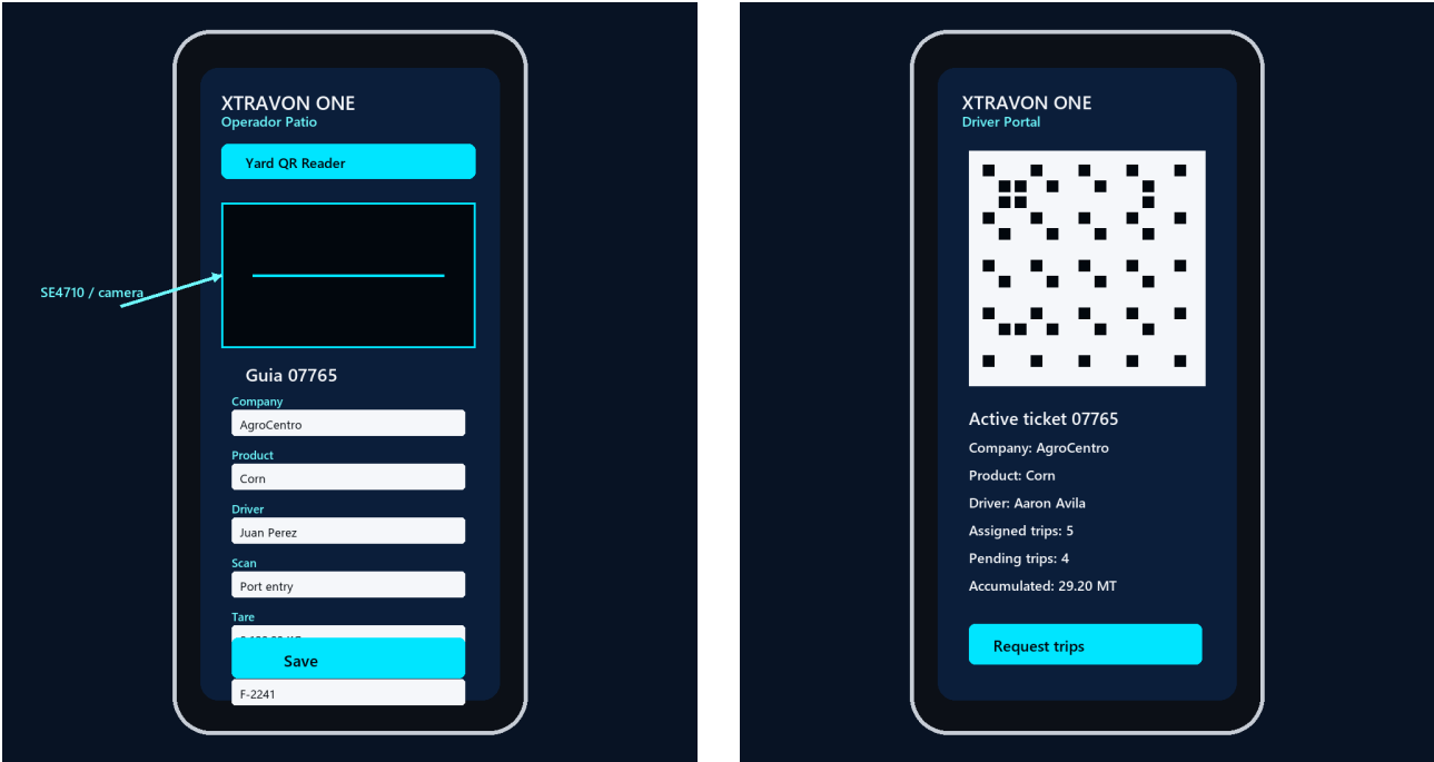
Yard handheld and driver portal: both must fit device margins and expose only the information required.
