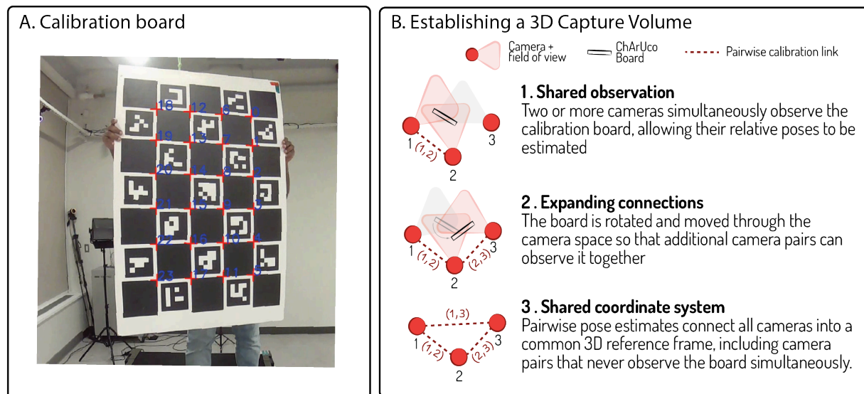
Figure 12. A. A ChArUco calibration board detected in a single video frame. Each ArUco marker has a unique identifier, allowing the intervening ChArUco corners to be detected and matched across images. The detected corner IDs are shown in blue. B. Establishing a shared 3D capture volume. When two or more cameras simultaneously observe the calibration board, their relative poses can be estimated. Moving and rotating the board through the capture space creates additional pairwise calibration links, progressively connecting all cameras into a common 3D reference frame, including camera pairs that do not directly observe the board at the same time.
