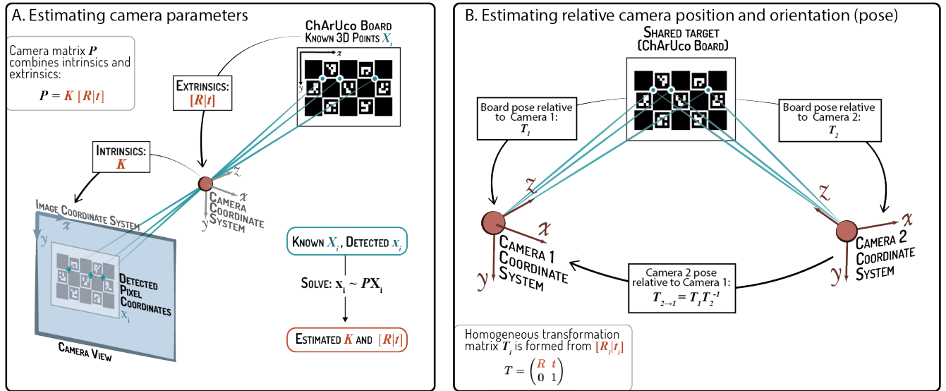
Figure 11. A. Estimation of camera intrinsic and extrinsic parameters using a ChArUco calibration board. Each ArUco marker has a unique identifier, allowing the intervening chessboard corners to be detected and assigned known locations within the board coordinate system. The board origin is defined at the first ChArUco corner, and the 3D coordinates of the remaining corners are determined from the known printed square size. Across multiple views of the board, correspondences between these known 3D corner locations, ( X_i ), and their detected 2D pixel coordinates, ( x_i ), are used to estimate the camera intrinsics, ( K ), and the board-to-camera extrinsics, ( [R|t] ). Together, these form the camera projection matrix ( P = K[R|t] ). B. Estimation of each camera’s position and orientation, collectively referred to as its pose, within a shared coordinate system. The extrinsic parameters estimated for each camera are first written as homogeneous transformation matrices, T_i . Camera 1 is then selected as the reference frame, and the pose of Camera 2 relative to Camera 1 is obtained by composing the two transforms: T_{2 \rightarrow 1} = T_1 T_2^{-1} . Repeating this process for the remaining cameras establishes the geometric relationships among all cameras in the system.
