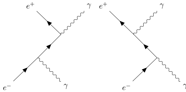
Figure 1: Electron-positron annihilation [1].
