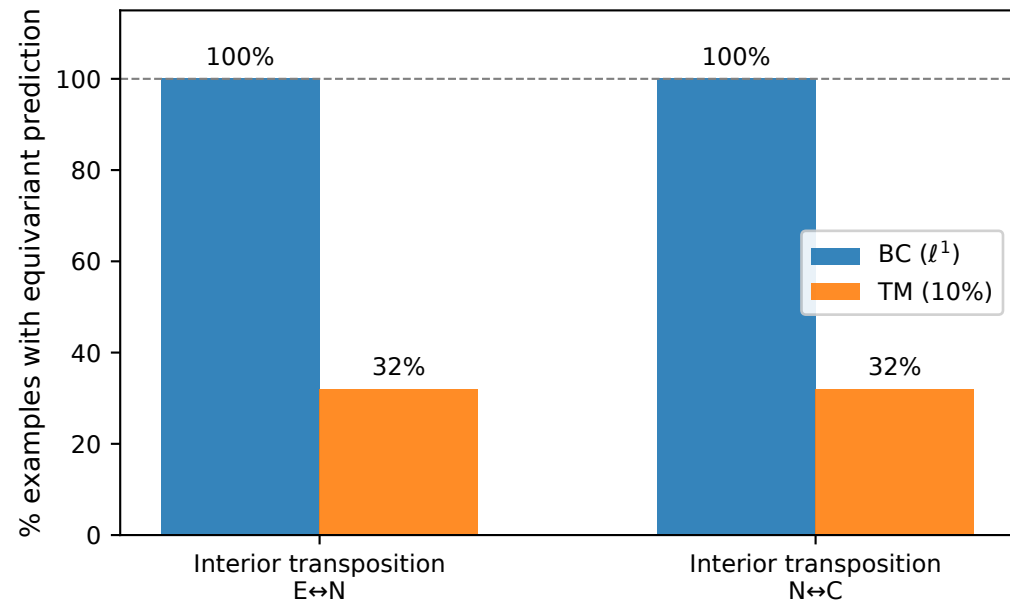
Permutation equivariance (100 random examples)
