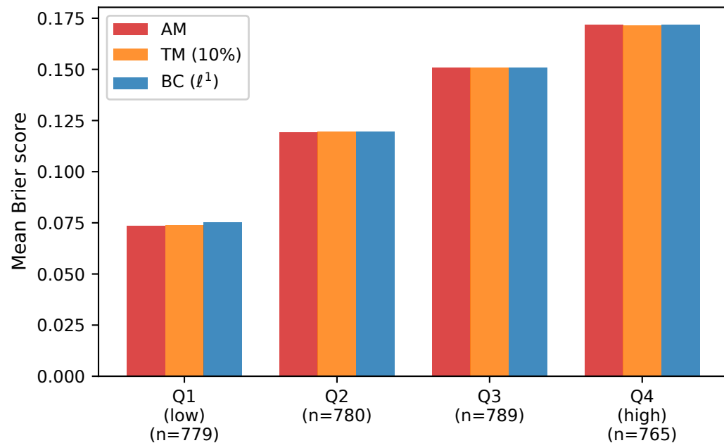
Mean Brier by panel dispersion (group-level ( n=10 ))
