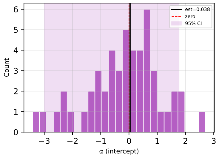
ECB8
