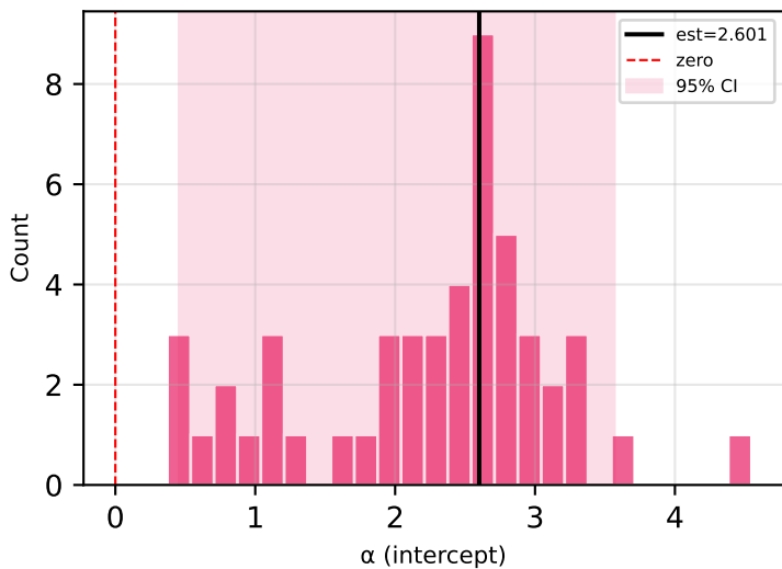
SPF-curr
