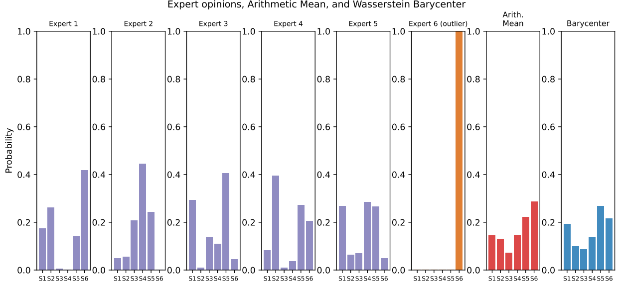
Figure 15: A single simulation draw: five regular experts (purple), one outlier (orange), arithmetic mean (red), and Wasserstein barycenter (blue). The arithmetic mean is visibly pulled toward the outlier’s distribution.
