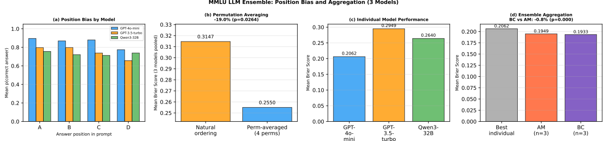
Figure 21: MMLU LLM ensemble results ( n = 3 models, K = 4 ). (a) Position bias by model: GPT models show 12–14pp gaps; Qwen3-32B shows only 1.7pp. (b) Effect of permutation averaging: BS 0.315 \rightarrow 0.255 (−19%, p = 0.026 ). (c) Individual model Brier scores. (d) Ensemble aggregation: BC 0.193 vs. AM 0.195 (−0.8%, p < 0.001 ).
