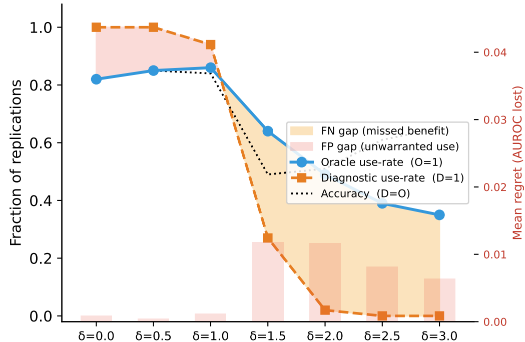
(a) Diagnostic vs oracle use-rate per \delta orange gap = FN (missed benefit) · red bars = regret
