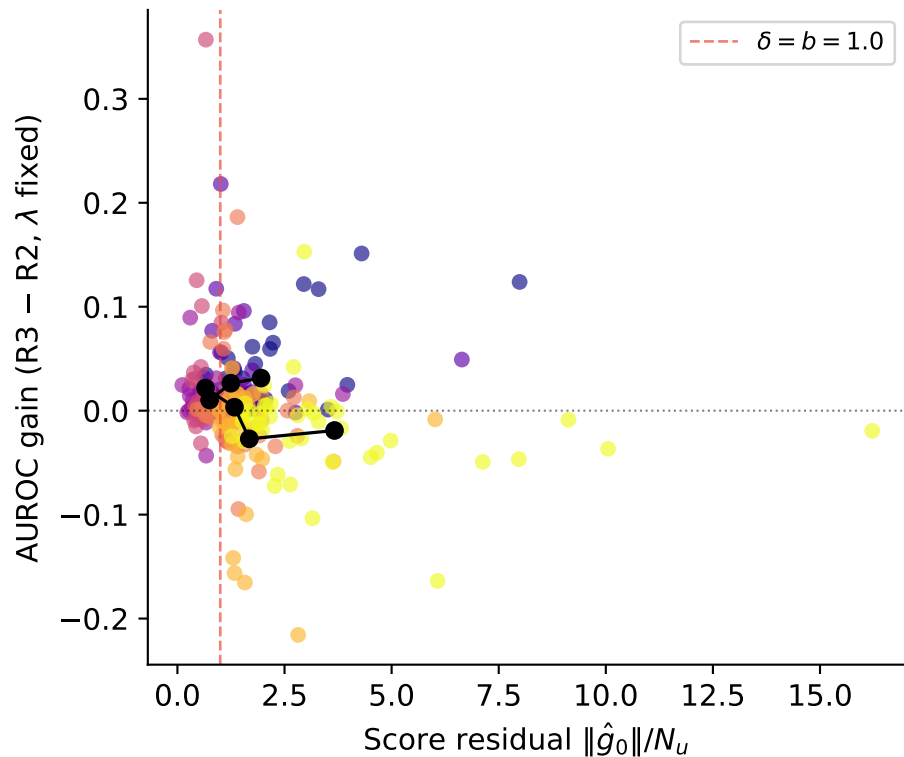
\|\hat{g}_0\|/N_u as pre-fitting risk indicator
