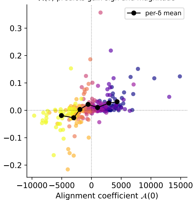
\mathcal{A}(0) predicts gain sign and magnitude
