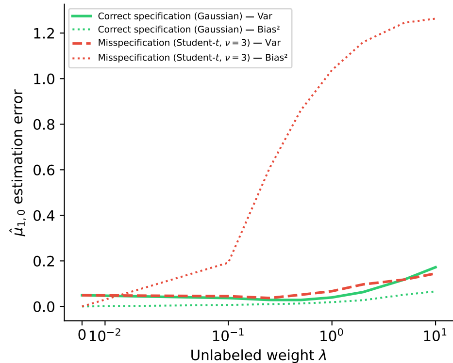
Variance \downarrow , Bias 2 \uparrow with \lambda
