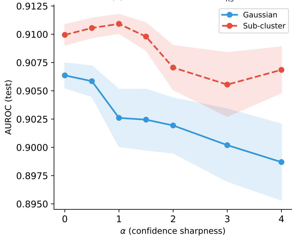
(b) R4: AUROC vs \alpha at \lambda = \lambda_{R3}^*
