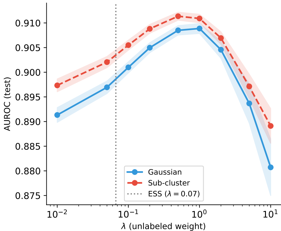
(a) R3: AUROC vs \lambda
