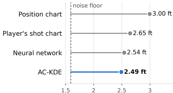
Mean shot-distance error
