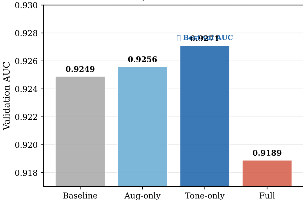
Figure 3. Ablation Study — Validation AUC All variants, HAM10000 validation set
