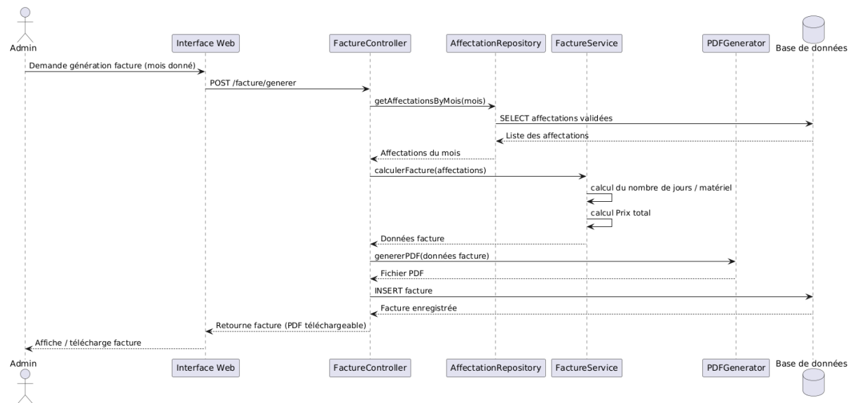
FIGURE 5 : DIAGRAMME DE SEQUENCE FACTURATION
