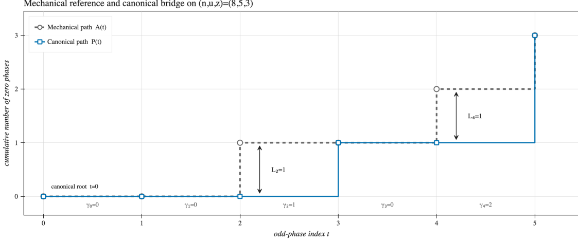
Figure 1: The exact mechanical path A and canonically rooted cumulative zero path P for w = 11101100 . Both are step interpolations of integer-valued data. They coincide at t = 0 and t = 5 , and their exact vertical separation is L_t = A(t) - P(t) . Together with the mechanical increments, the successive differences of L recover the zero gaps.
