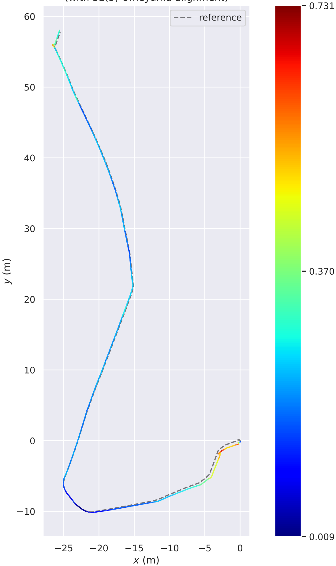
APE w.r.t. translation part (m) (with SE(3) Umeyama alignment)
