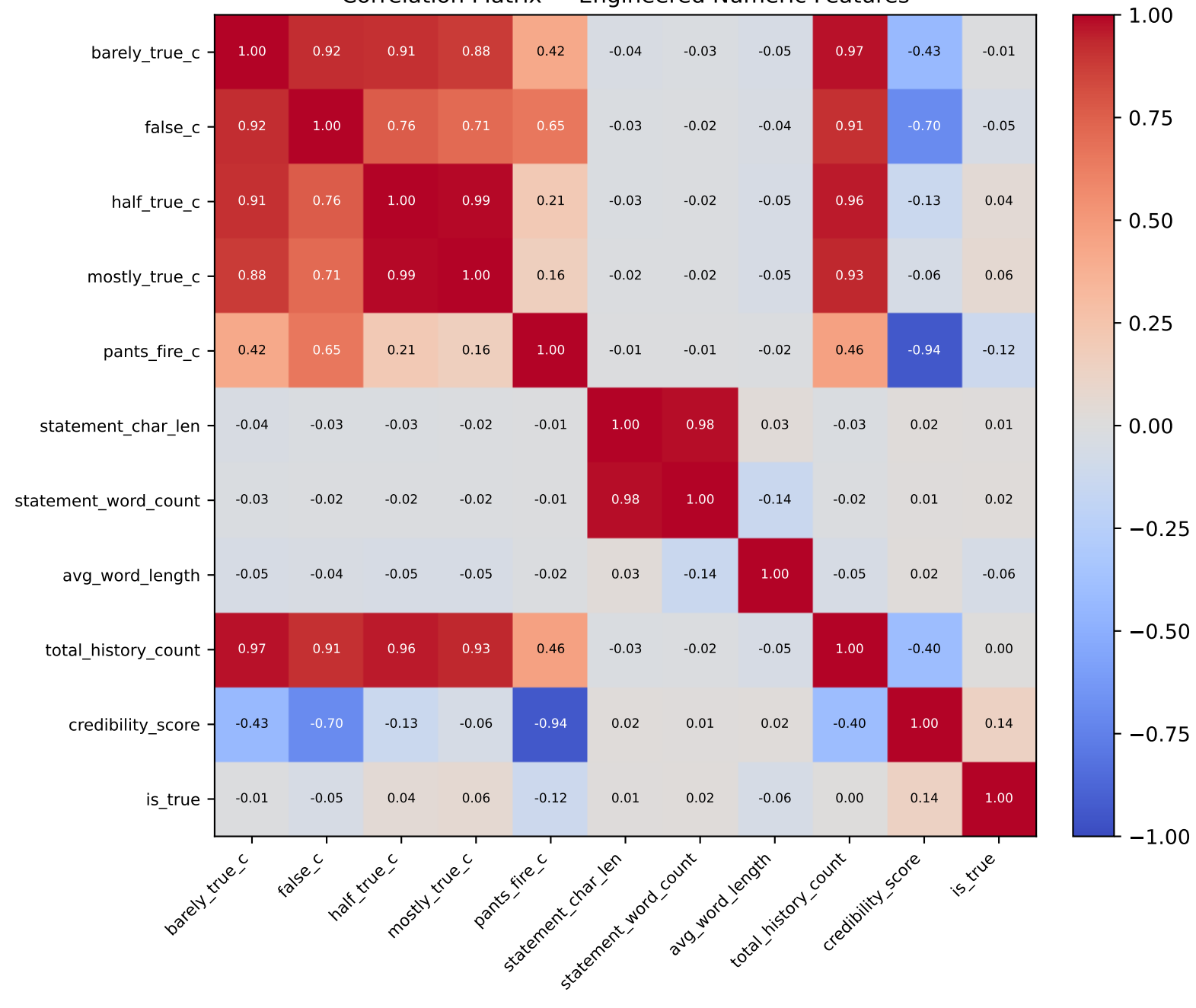
Correlation Matrix — Engineered Numeric Features
