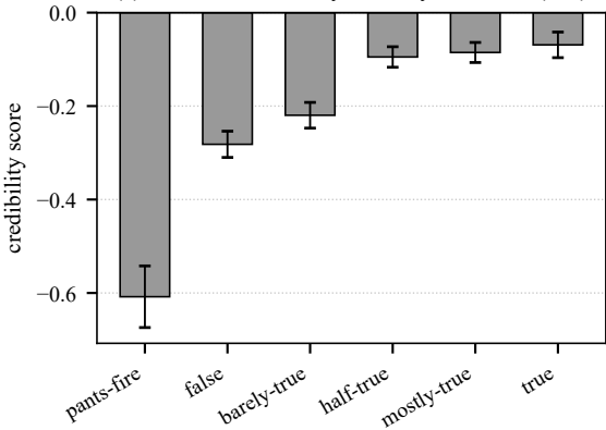
(a) leak-free credibility score by true label (test)
