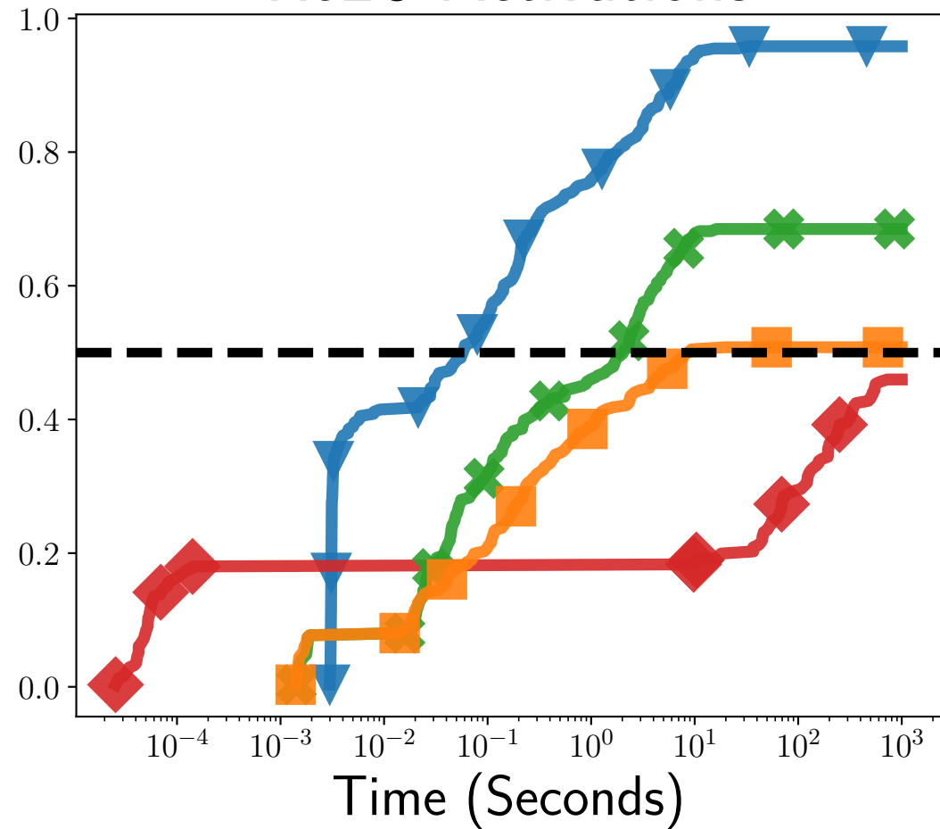
ReLU Activations
