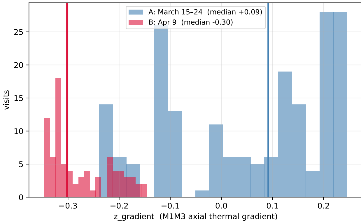
M1M3 axial thermal gradient by epoch
