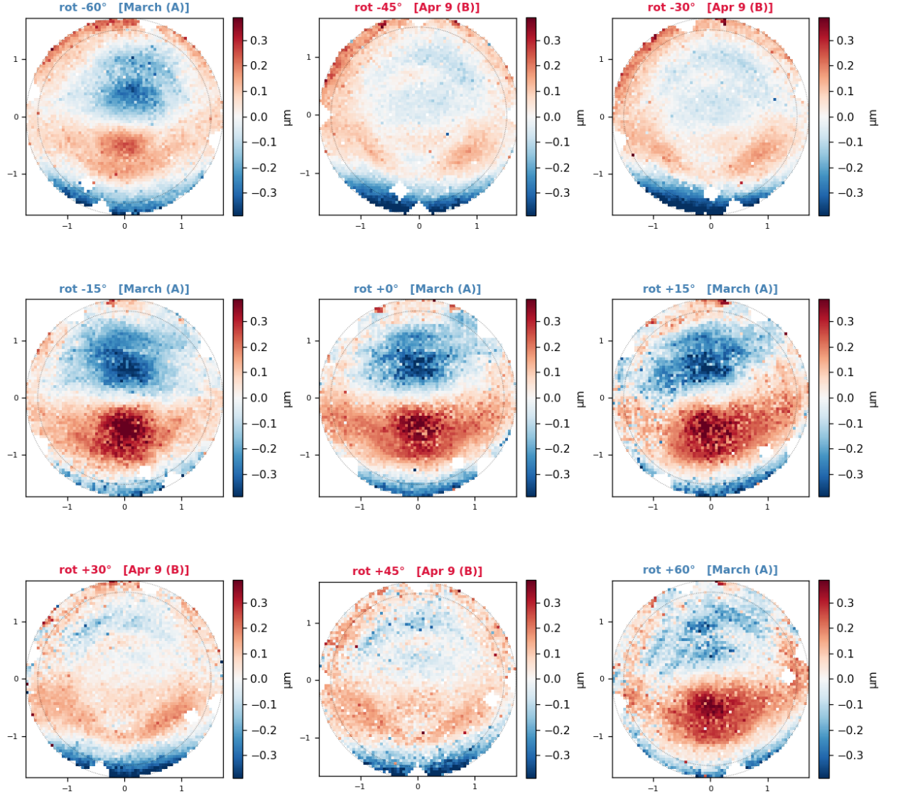
Z7 coma measured intrinsic by rotator angle (fam_danish_1_0_wep17_3_0_bin2x / pathA_50_34_i) blue = March epoch (A); red = Apr-9 epoch (B) — the \pm 30/\pm 45 maps are the second family
