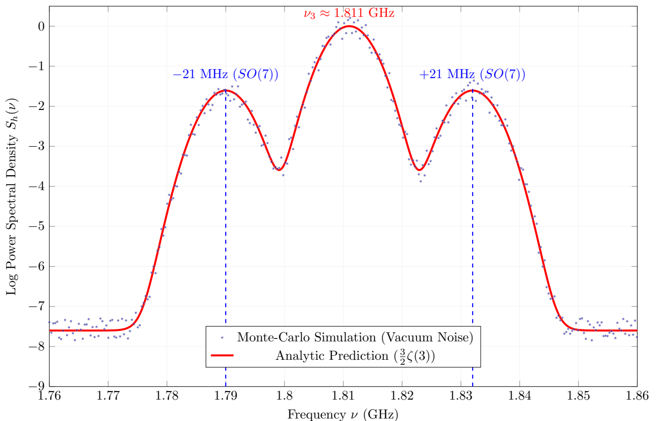
Figure 2: Spectral Profile of the Sedenion Scream. The red curve represents the analytic prediction derived from the \zeta(3) entropic capacity of the S^3 fibers, anchored to the Hydrogen line. The grey data points represent a Monte-Carlo simulation of the stochastic gravitational wave background, incorporating Rule 30-class vacuum fluctuations. The distinct sidebands at \pm 21 MHz correspond to the relaxation of the SO(7) embedding dimensions.
