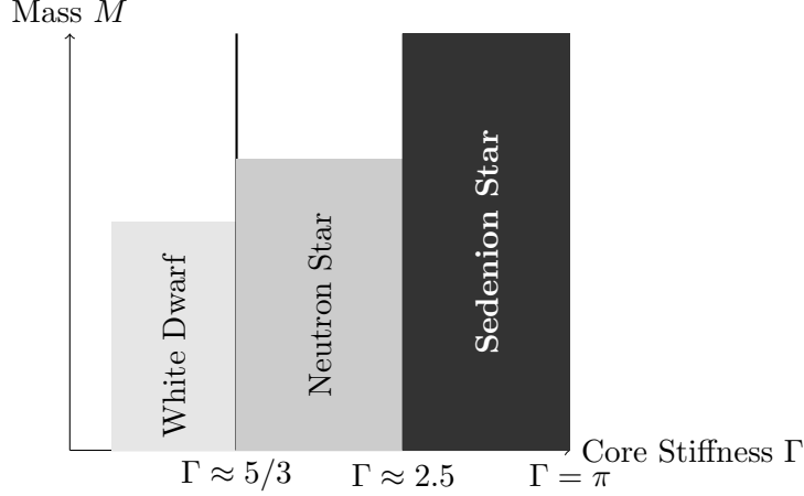
Figure 1: The APH Phase Diagram. The black hole is identified as the thermodynamic state where vacuum stiffness saturates at the geometric limit \pi .
