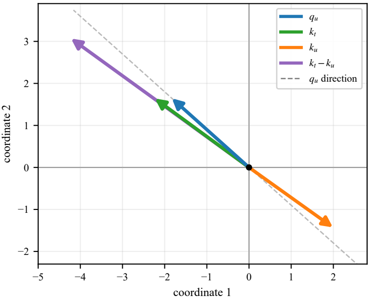
Learned query/key geometry
