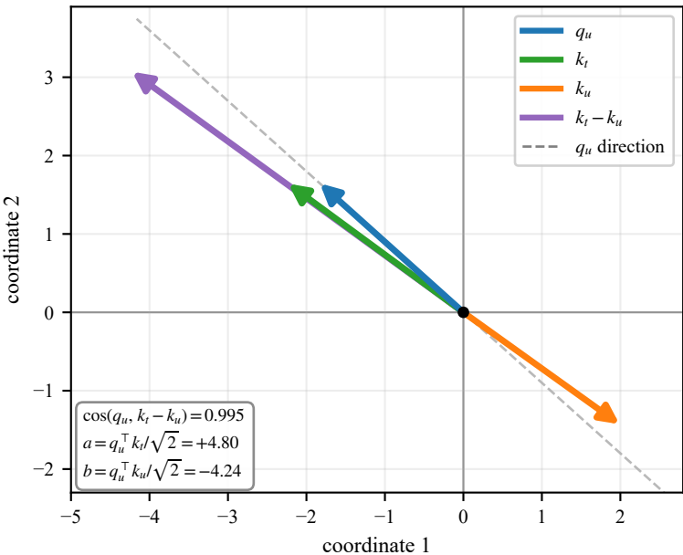
Learned query/key geometry (learned_log_e200, seed 1)
