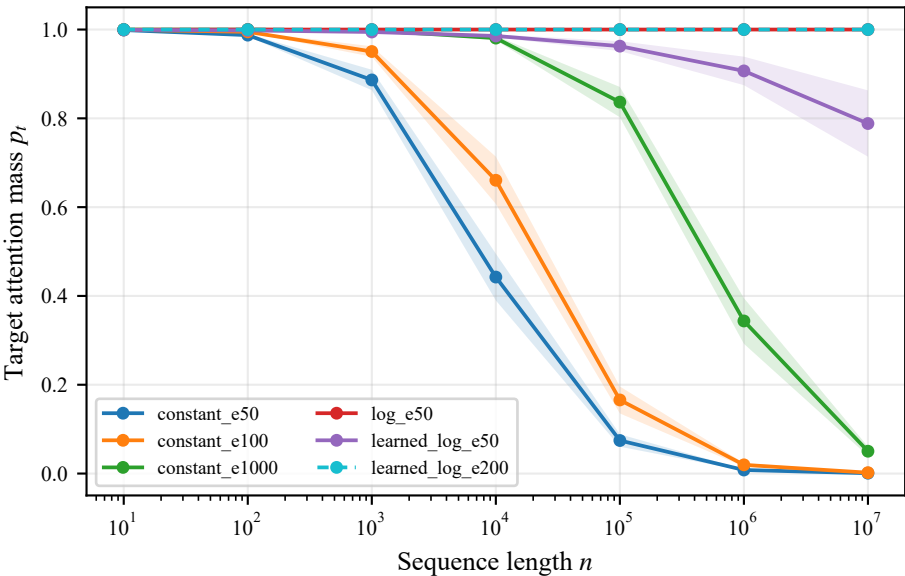
Target attention by sequence length
