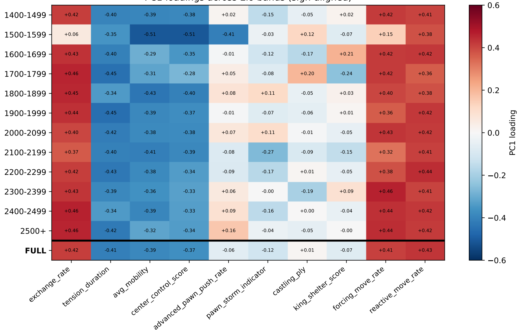
PC1 loadings across Elo bands (sign-aligned)
