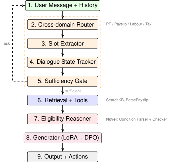
Figure 1: ShramikSaathi pipeline. Orange layers form the pre-retrieval pipeline; the eligibility reasoner (red) is the core novel component. Dashed arrow indicates the ask-loop when slots are insufficient.
