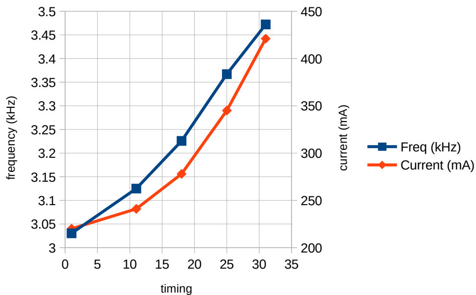
Remora with unloaded 3000Kv motor, rotation frequency & current vs timing
