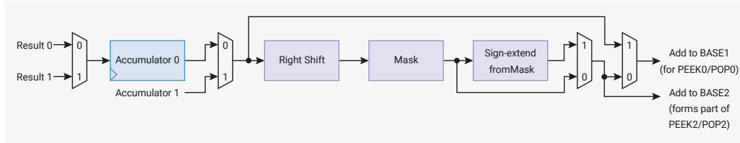
Figure 9. Each lane of each interpolator can be configured to perform mask, shift and sign-extension on one of the accumulators. This is fed into adders which produces final results, which may optionally be fed back into the accumulators with each read. The datapath can be configured using a handful of 32-bit multiplexers. From left to right, these are controlled by the following CTRL flags: CROSS_RESULT, CROSS_INPUT, SIGNED, ADD_RAW.
