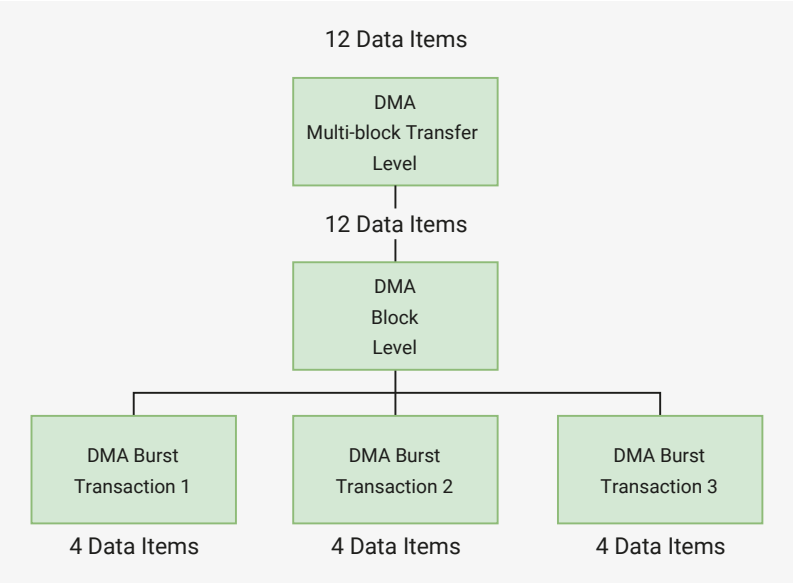
Figure 164. Breakdown of DMA Transfer into Burst Transactions. Block size, DMA.CTLx.BLOCKS_TS = 12. Number of data items per source burst transaction, DMA.CTLx.SRC_MSIZ = 4. SSI receive FIFO watermark level, SSI.DMATDLR + 1 = DMA.CTLx.SRC_MSIZ = 4
