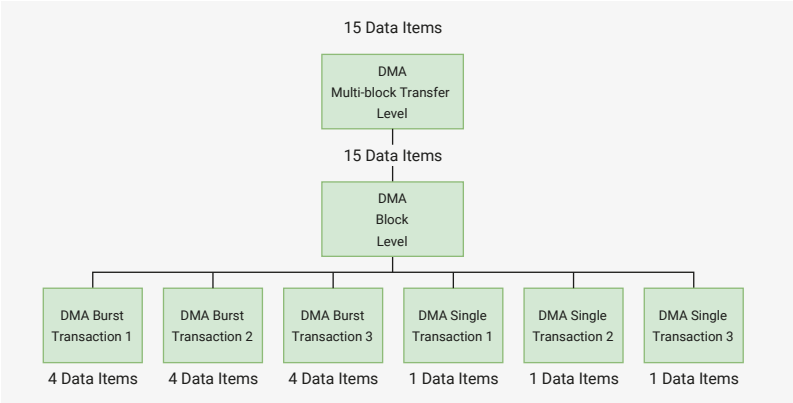
Figure 165. Breakdown of DMA Transfer into Single and Burst Transactions. Block size, DMA.CTLx.BLOCK_TS = 15. Number of data items per burst transaction, DMA.CTLx.DEST_MSIZ = 4. SSI transmit FIFO watermark level, SSI.DMATDLR = DMA.CTLx.DEST_MSIZ = 4
