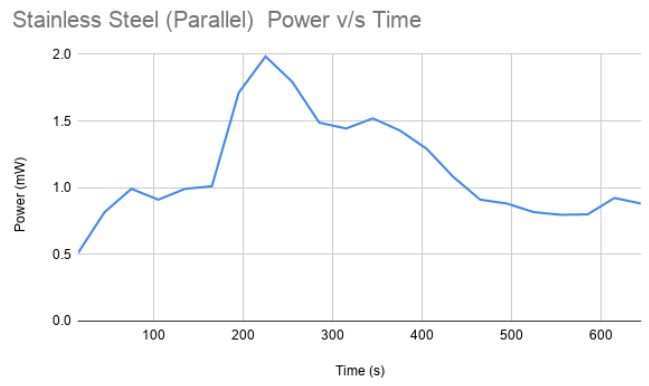
Fig. 8. Power vs. Time: stainless-steel plates connected in parallel
