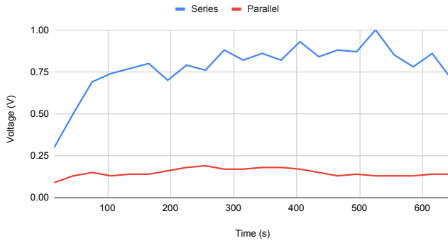
Series and Parallel (Stainless Steel) Voltage v/s Time
