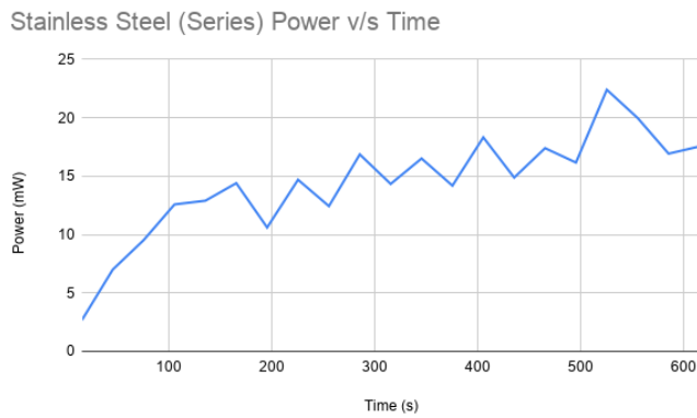
Fig. 5. Power vs. Time: stainless-steel plates connected in series
