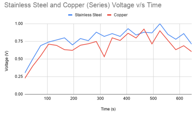
Fig. 12. Voltage vs. Time: comparison between stainless-steel and copper plates in series
