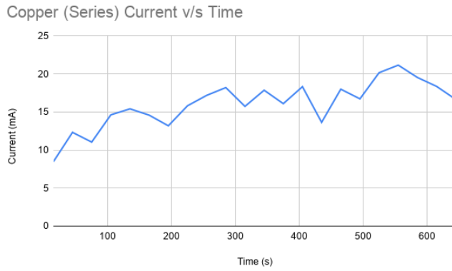
Fig. 10. Current vs. Time: copper plates connected in series
