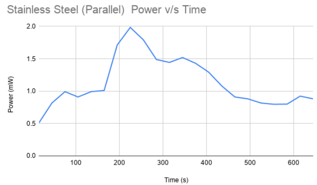
Fig. 8. Power vs. Time: stainless-steel plates connected in parallel
