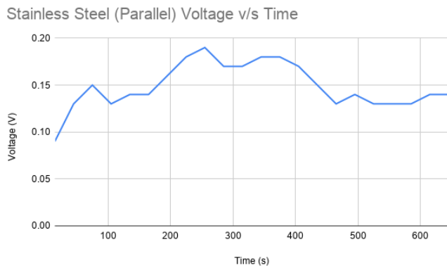
Fig. 6. Voltage vs. Time: stainless-steel plates connected in parallel
