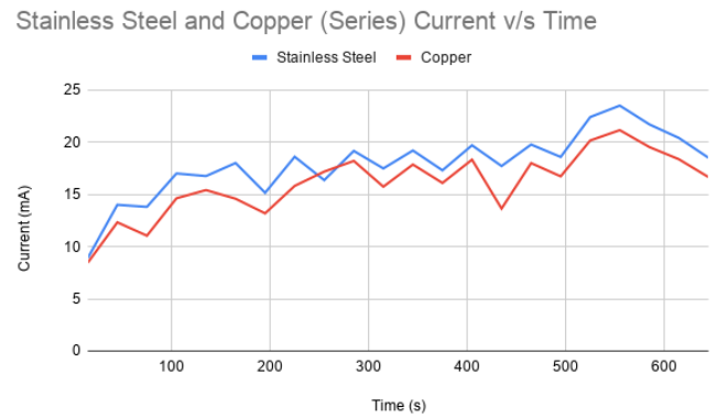
Fig. 13. Current vs. Time: comparison between stainless-steel and copper plates in series
