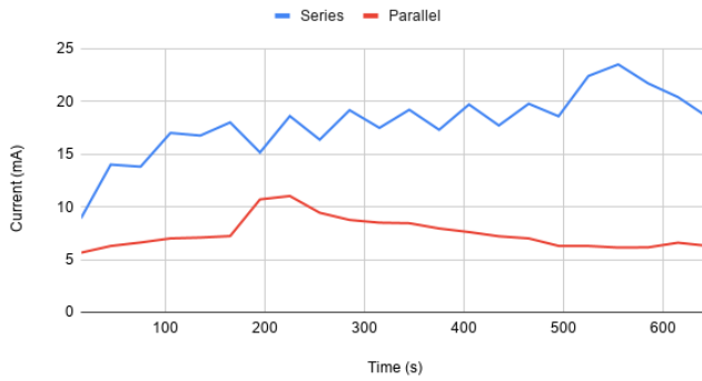
Series and Parallel (Stainless Steel) Current v/s Time
