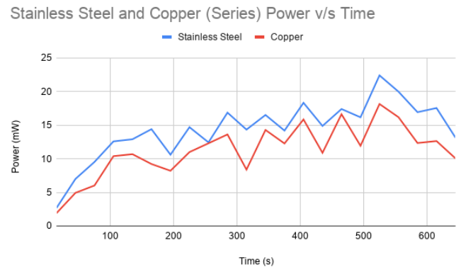
Fig. 14. Power vs. Time: comparison between stainless-steel and copper plates in series
