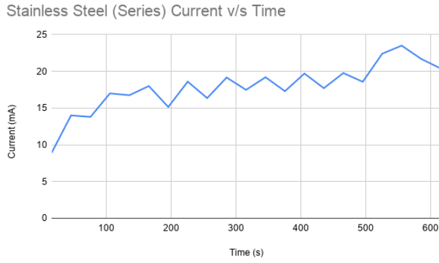
Fig. 4. Current vs. Time: stainless-steel plates connected in series
