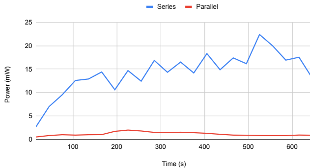
Series and Parallel (Stainless Steel) Power v/s Time
