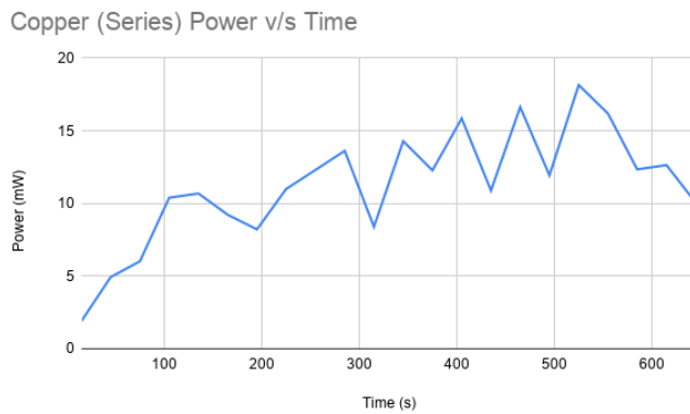
Fig. 11. Power vs. Time: copper plates connected in series
