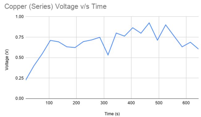
Fig. 9. Voltage vs. Time: copper plates connected in series
