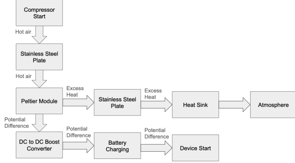
Fig. 1. AC compressor as thermoelectric heat generator
