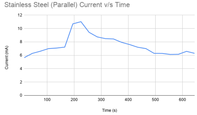
Fig. 7. Current vs. Time: stainless-steel plates connected in parallel
